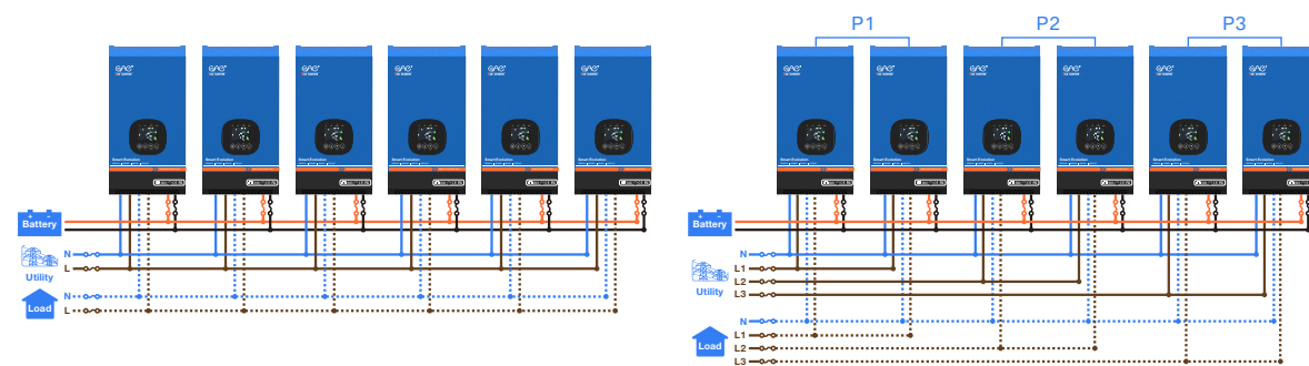
Parallel Operation in Single phase
